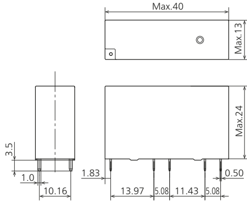
External dimensions
