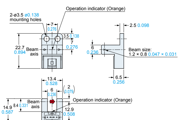
PM-Y65 PM-Y65-P Sensor
