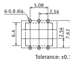
Recommended mounting pad (TOP VIEW)
