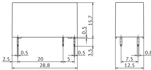
External dimensions
