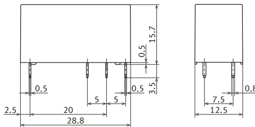
External dimensions
