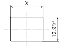
P/C board pattern
