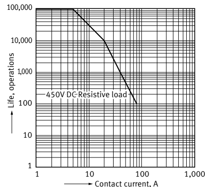
3. Switching life curve
