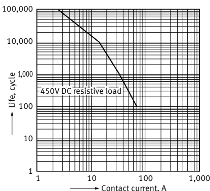
3. Switching life curve (Forward direction)
