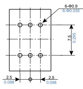
Recommended PC board pattern (TOP VIEW)
