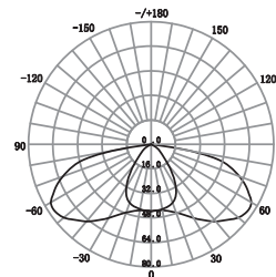
EMD Narrow Lens (Path Way) EMD Fluchtwegoptik
