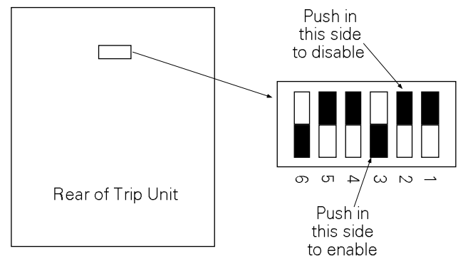
Figure 5. Accessory switch on the rear of a MicroVersaTrip Plus™ or MicroVersaTrip PM™ Trip Unit, showing the factory settings (solid part indicates that switch is pushed in on that side).
