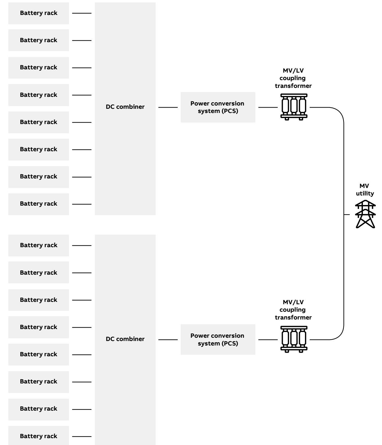
Example of 4 MWh BESS
