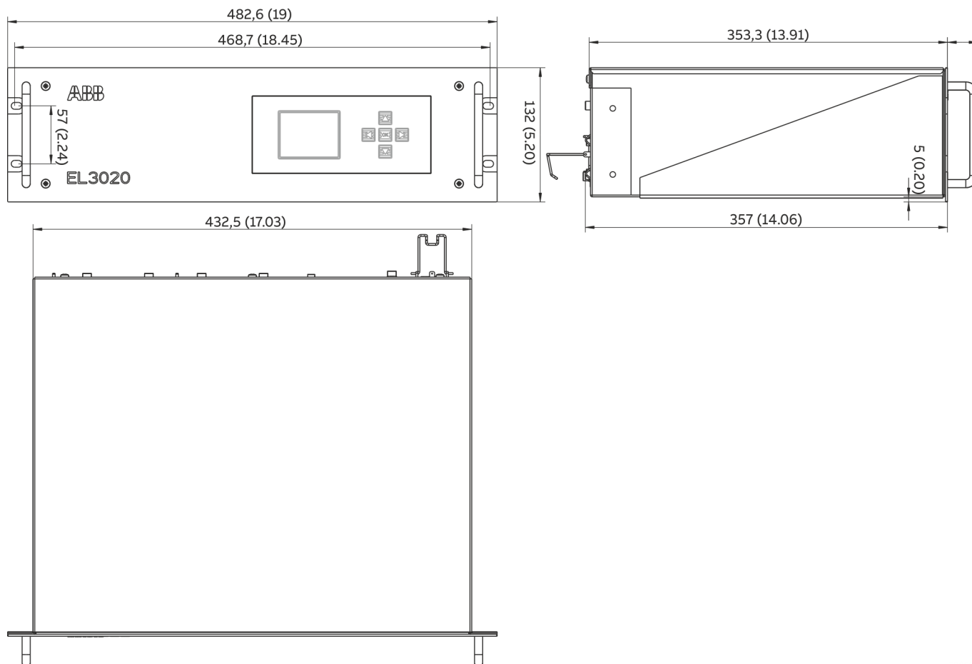
Figure 3: 19" housing (model EL3020)
