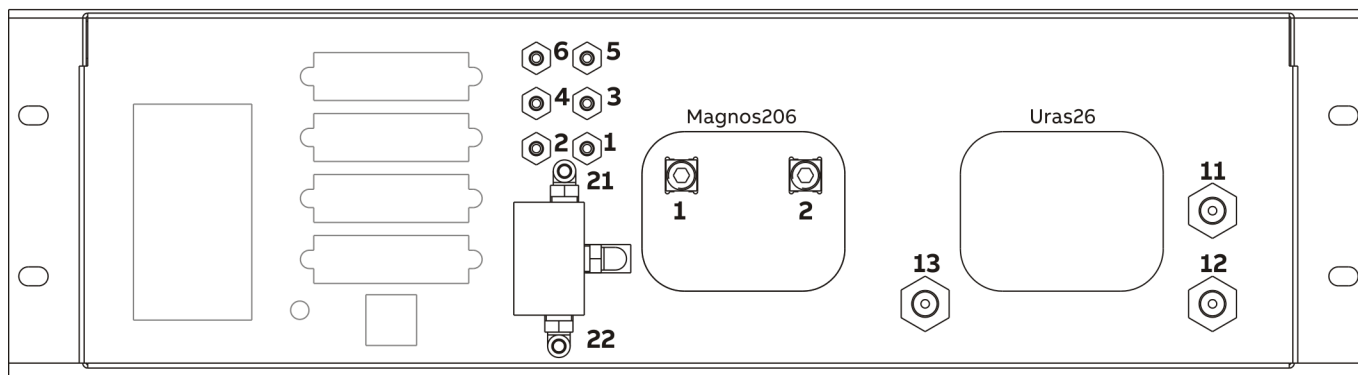
Figure 8: Gas connections Uras26 with Magnus206 (model EL3020)
