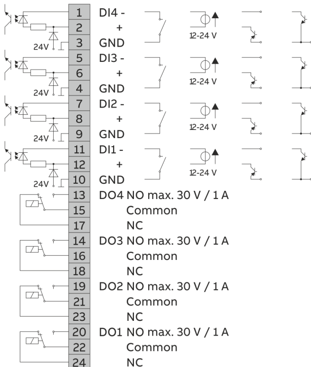
Figure 44: Electrical connections, digital I/O module
