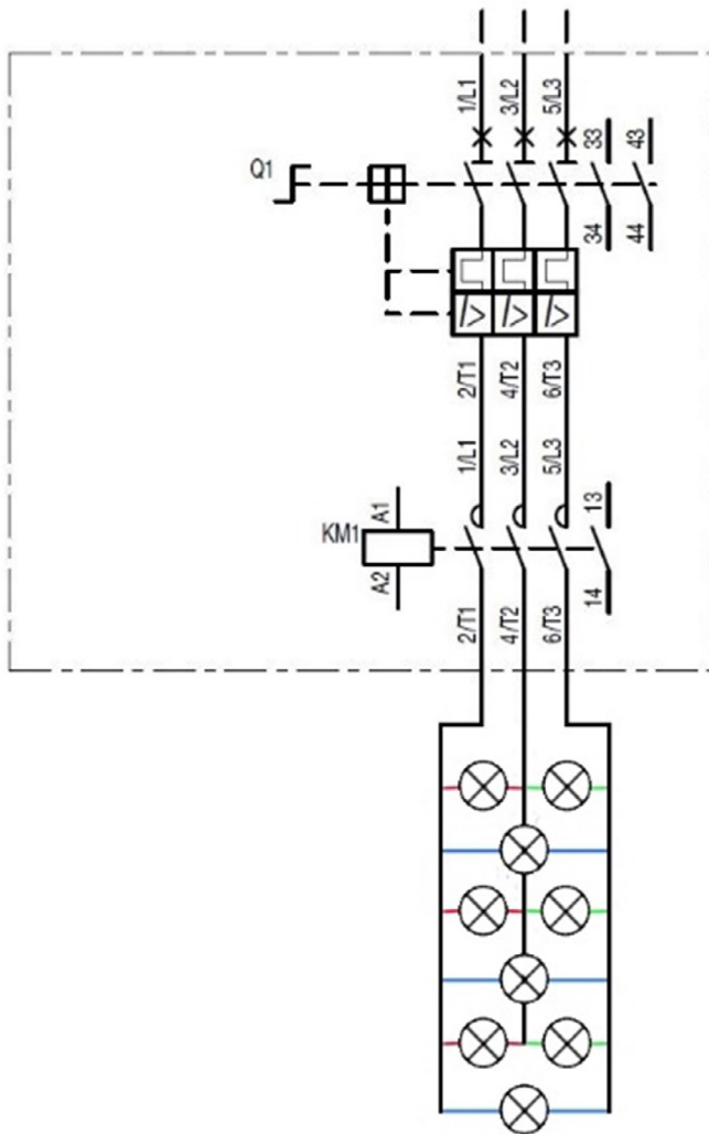
12 Lamp starter in power circuit with lamp loads
