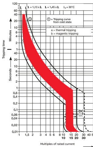
D characteristic
