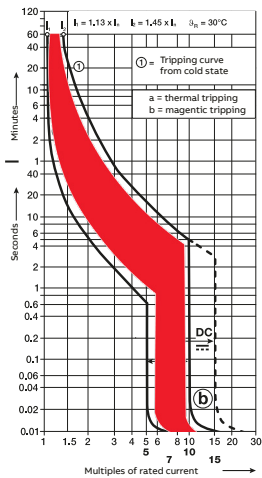
C characteristic
