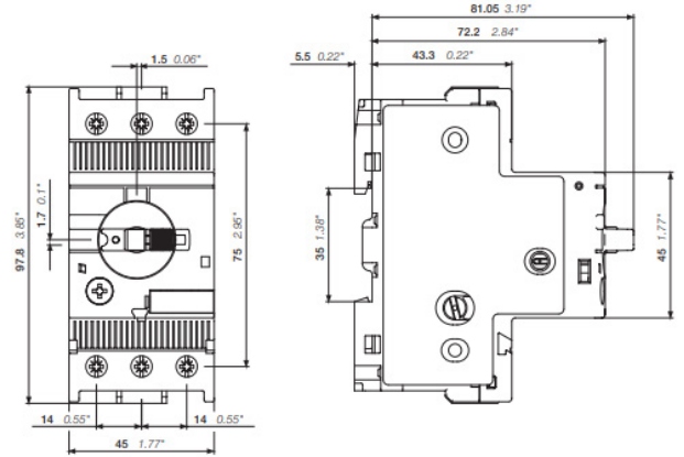
14 MS132-10LC
