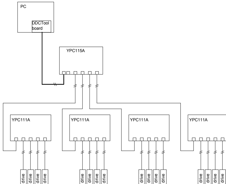
Figure 2 - 4. The tree form of one YPC115A and four YPC111As.
