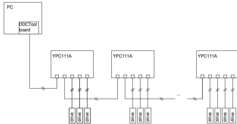
Figure 2 - 1. Chain form of the YPC111A optical distributor. When using plastic fibre cable the maximum length is 20 metres.
