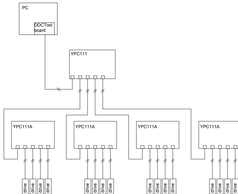
Figure 2 - 2. Tree form of the YPC111A optical distributor. When using plastic fibre cable the maximum length is 20 metres.
