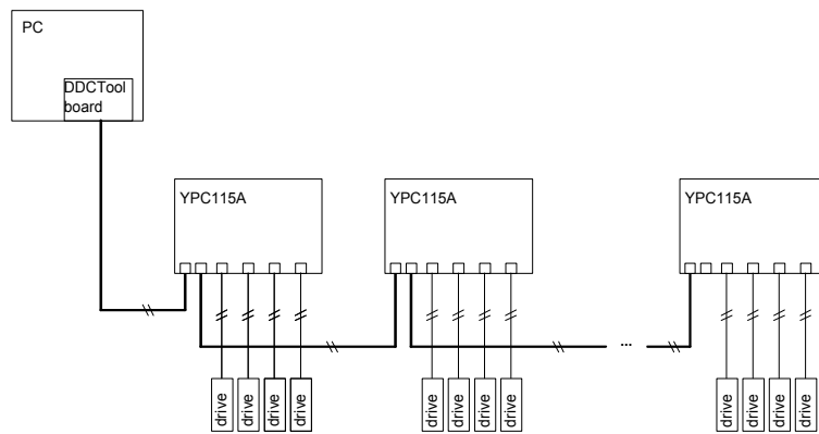
Figure 2 - 3. The chain form of the YPC115A. When using glass fibre cable the maximum length is 1000 metres (the dark lines).
