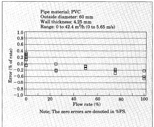
Fig. 6 Measurement error
