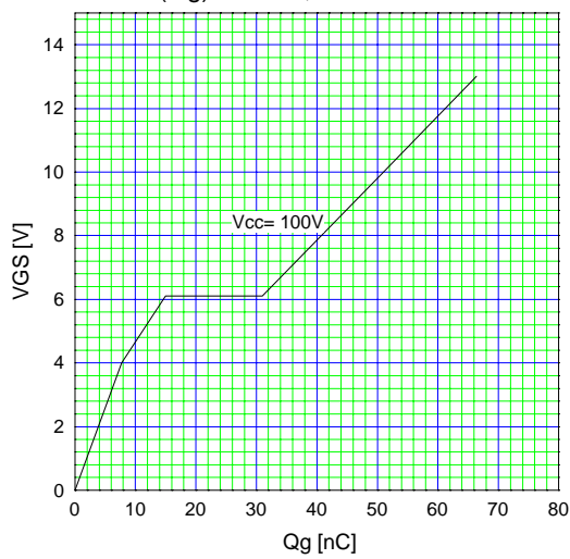
Typical Gate Charge Characteristics V_{GS}=f(Q_g):I_D=30A, T_{ch}=25^\circ C
