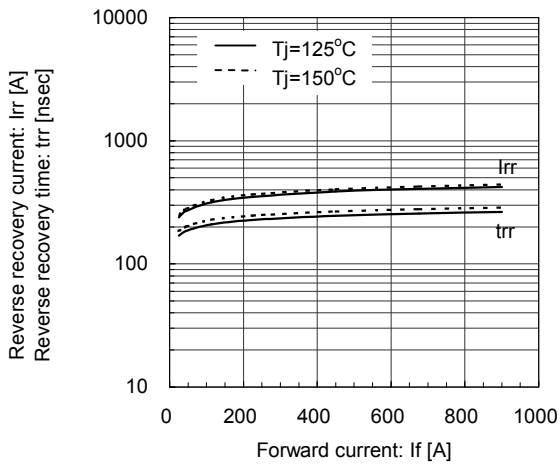
Reverse Recovery Characteristics (typ.) Vcc=600V, Vge=±15V, Rg=0.52Ω, Tj=125°C, 150°C
