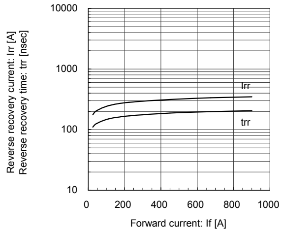
Reverse Recovery Characteristics (typ.) Vcc=600V, Vge=±15V, Rg=0.52Ω, Tj=25°C
