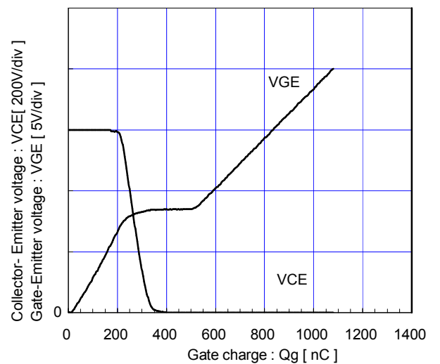
Dynamic Gate charge (typ.) Vcc=600V, Ic=225A, Tj=25°C
