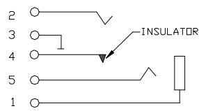
CIRCUIT SCHEMATIC
